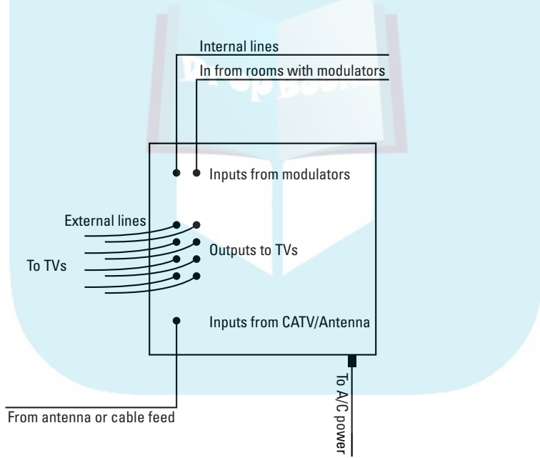
Figure 6-7: The distribution panel is the center of a video network.
